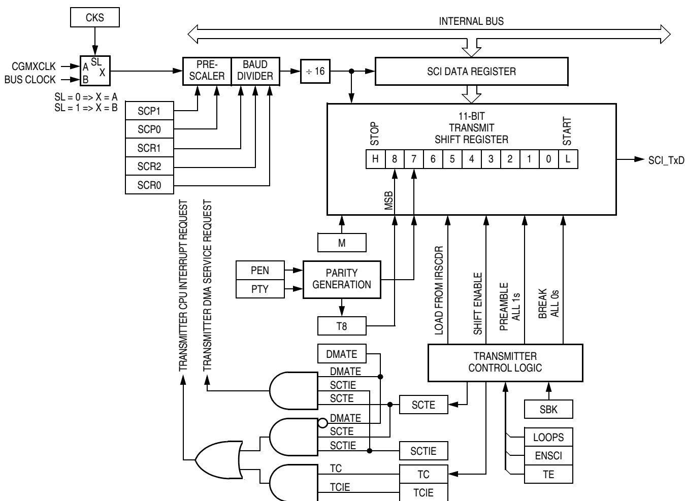
Figure 14-7. SCI Transmitter
