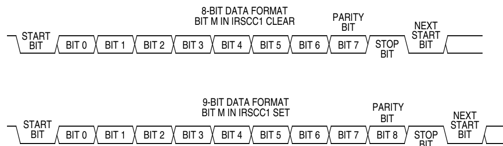
Figure 14-6. SCI Data Formats
