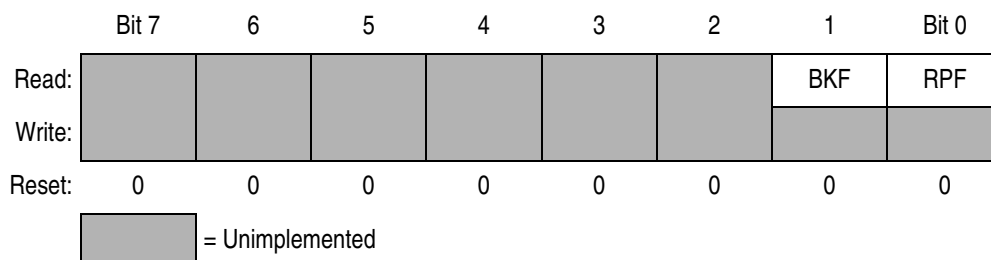
Figure 13-14. SCI Status Register 2 (SCS2)
