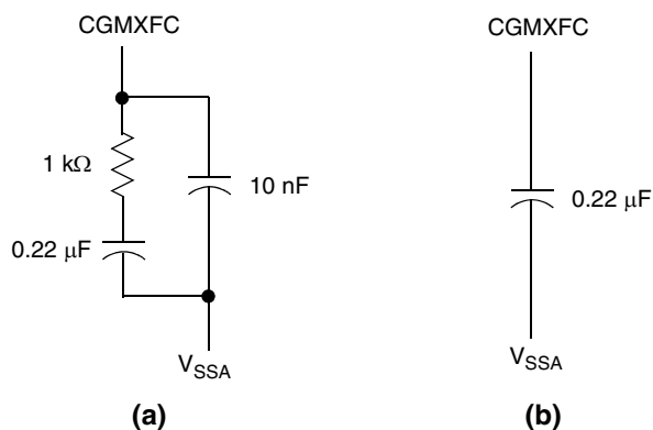
Figure 8-10. PLL Filter
