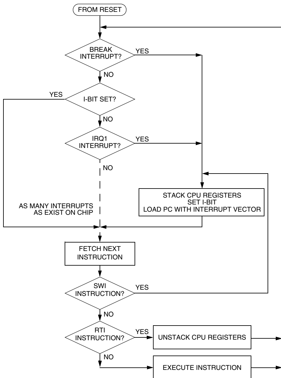
Figure 9-10. Interrupt Processing
