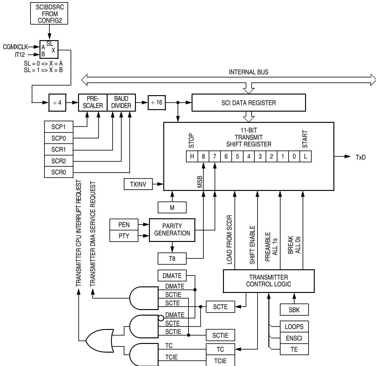
Figure 13-4. SCI Transmitter
