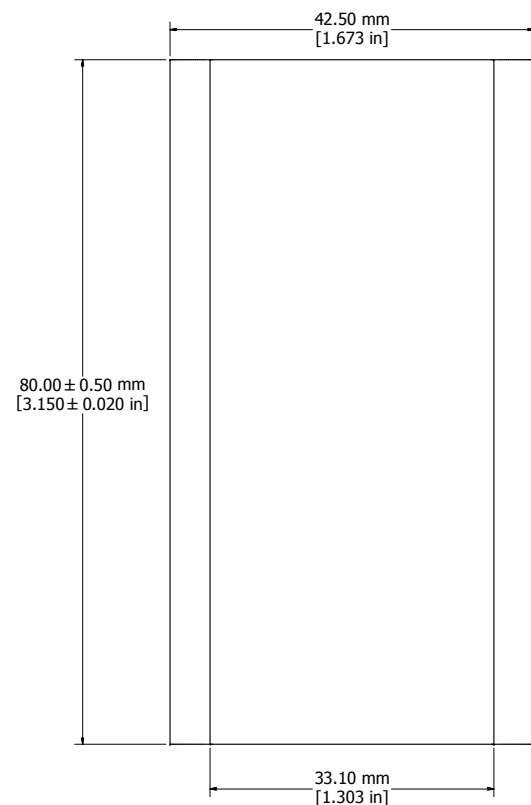
EXTRUSION PROFILE
