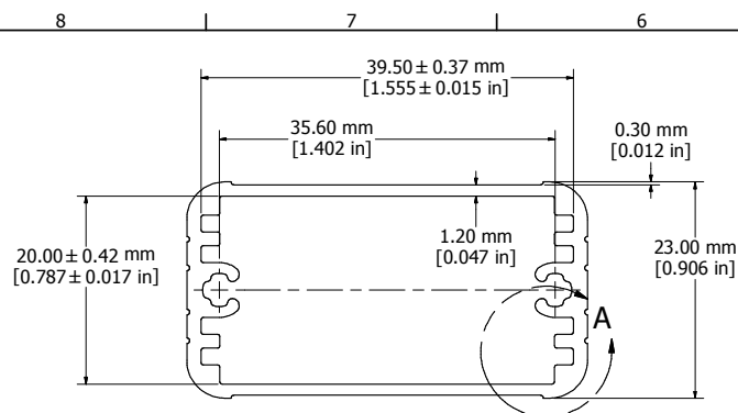
EXTRUSION PROFILE
