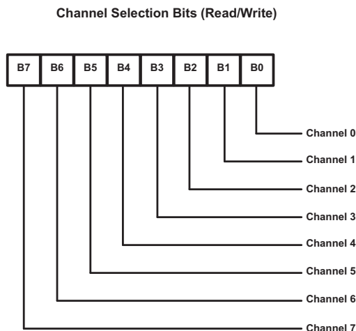
Figure 7. Control Register
