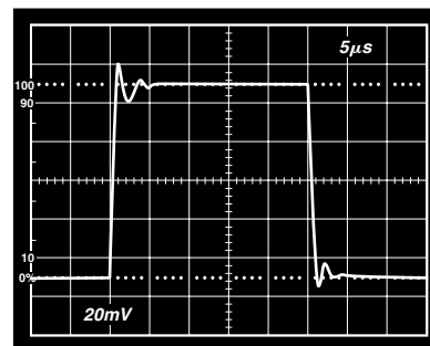
TPC 21d. Unity Gain Inverter Small Signal Pulse Response, C_L = 1,000 pF
