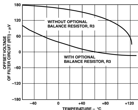
Figure 5. V_{OS} vs. Temperature Performance of the 1 Hz Filter Circuit
