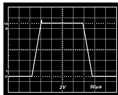
TPC 20b. Unity Gain Follower Large Signal Pulse Response R_F = 10 \text{ k}\Omega , C_L = 1,000 \text{ pF}
