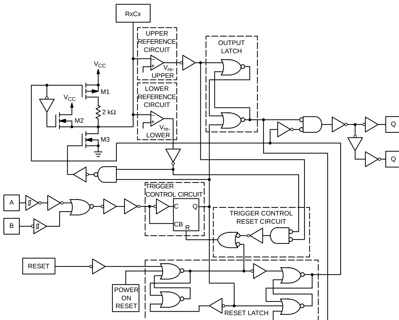
Figure 11. Logic Detail (1/2 the Device)
