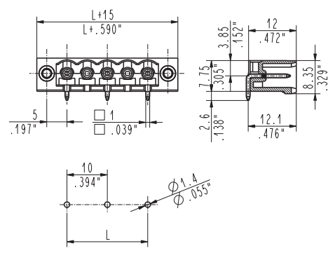
CIM_5V2 270°, locking screw flanges male
