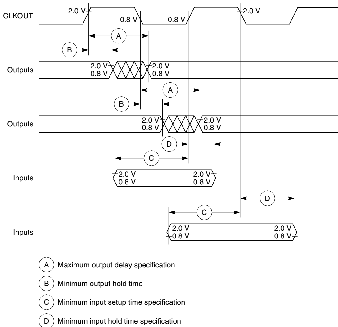
Figure 3. Control Timing
