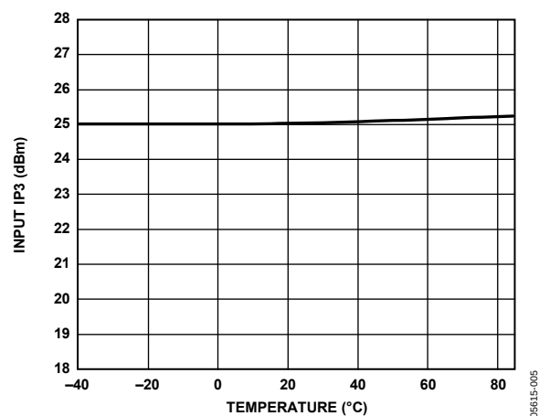
Figure 5. Input IP3 (IIP3) vs. Temperature
