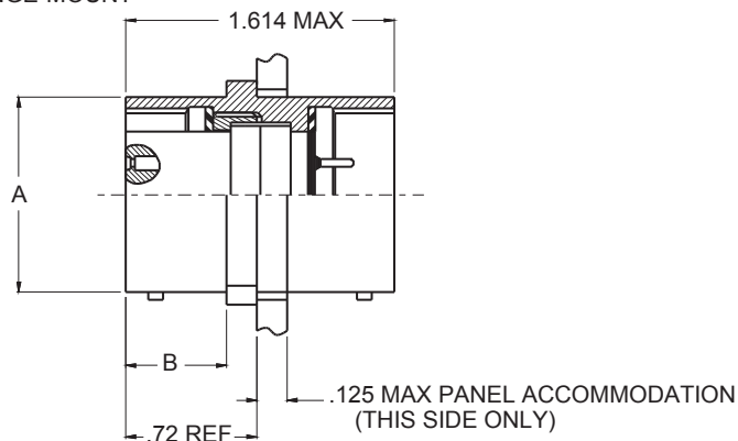
STYLE B FLANGE-MOUNT
