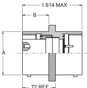
STYLE A IN-LINE
