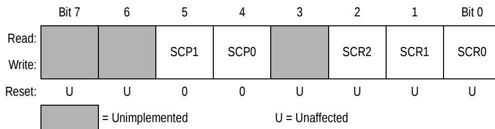
Figure 10-9. Baud Rate Register (Baud)
