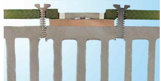
Sectional view shows sandwich of ACULED with TL-PCB mounted on standard heat sink
