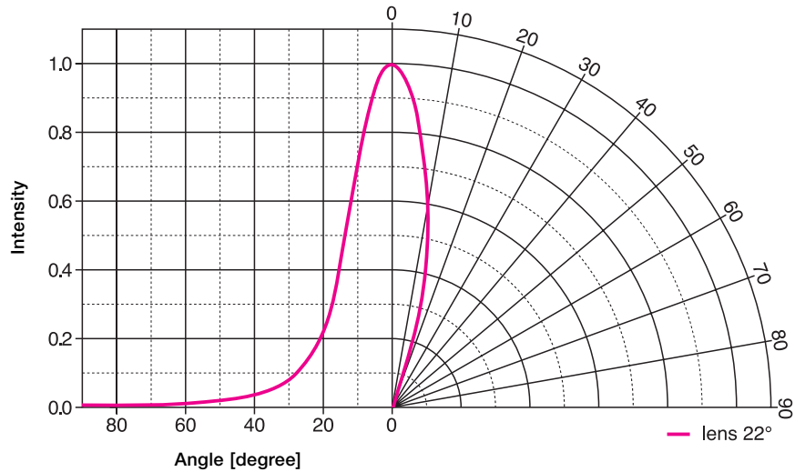
Opening Angle: Example RGB with Lens
