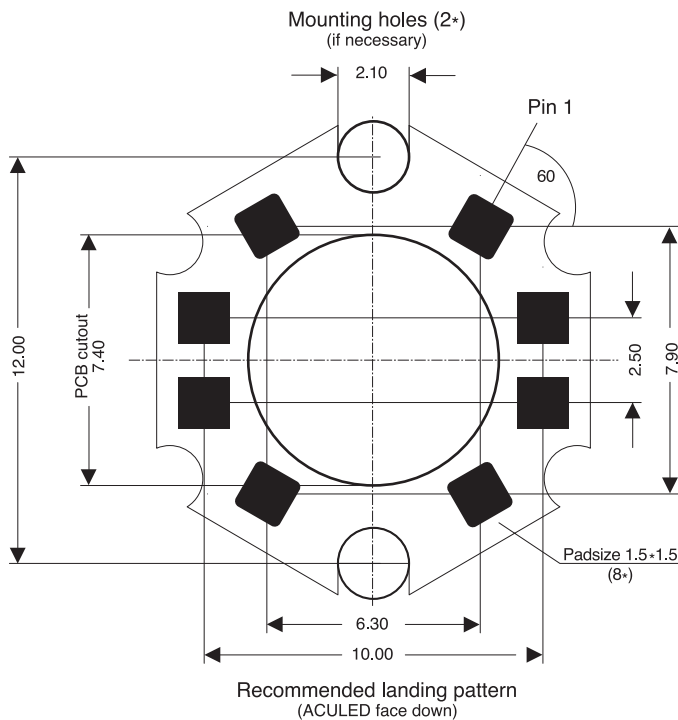
Recommended Solder Pad Geometry
