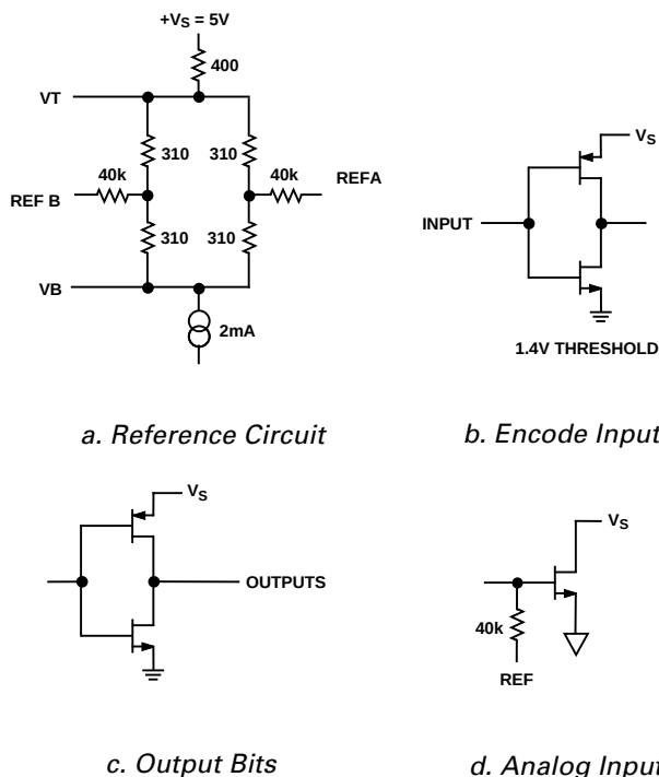
Figure 4. Equivalent Circuits
