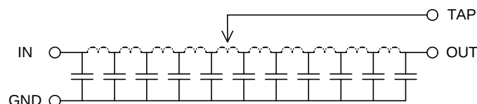
Functional Diagram
