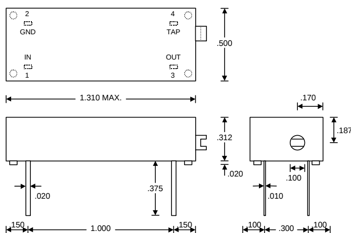
Package Dimensions - 1503
