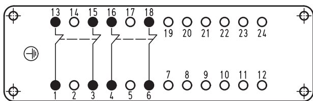
Schaltplan/wiring diagram
