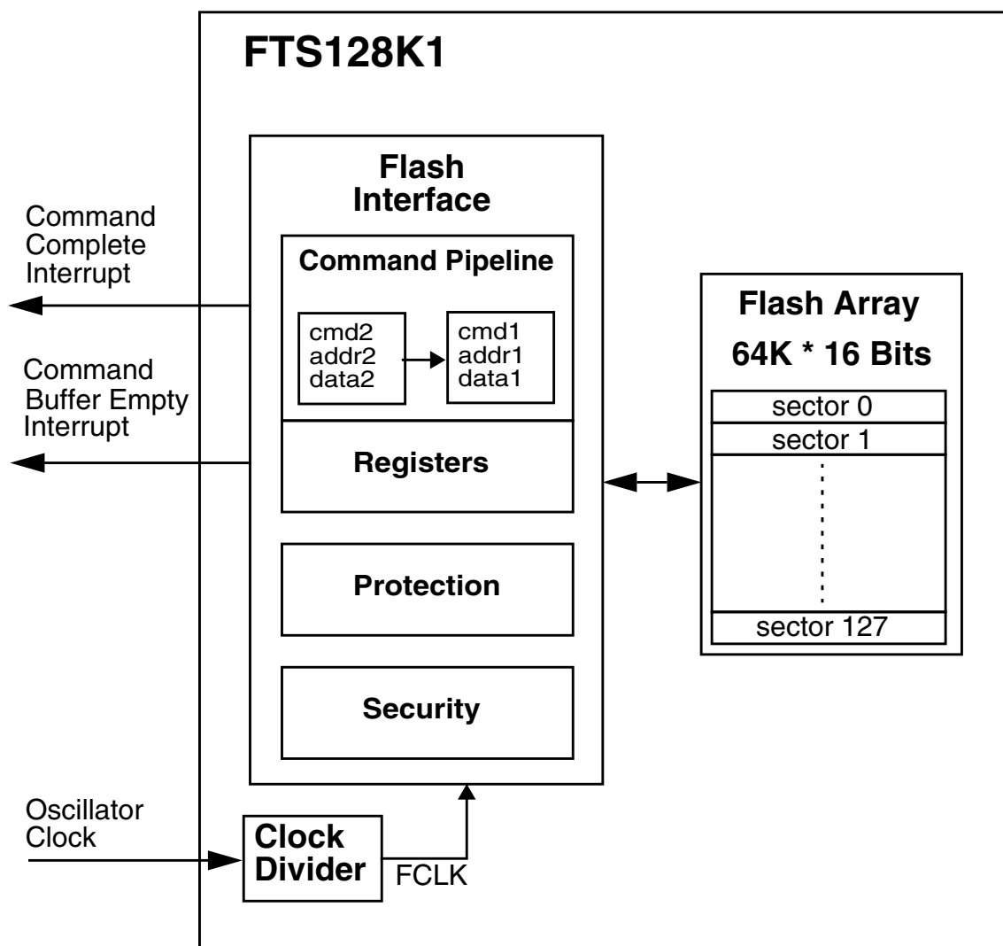
Figure 19-1. FTS128K1 Block Diagram
