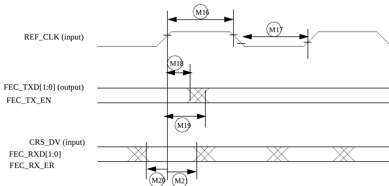
Figure 59. RMII Mode Signal Timing Diagram
