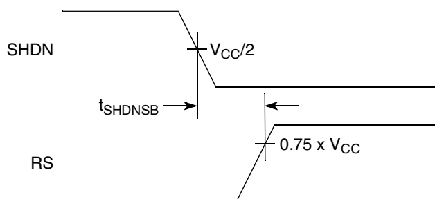
Figure 63. Timing Diagram for FlexCAN Shutdown-to-Standby Signal
