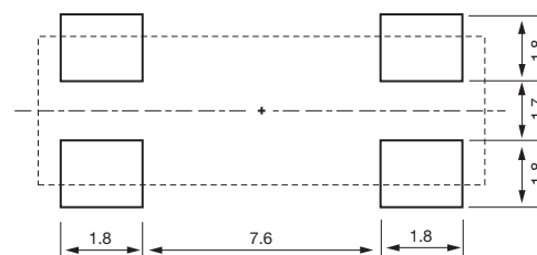
Figure 4) ECX-3S Land Pattern - Bottom view
