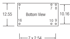
16 Pin Mini-DIP Package
