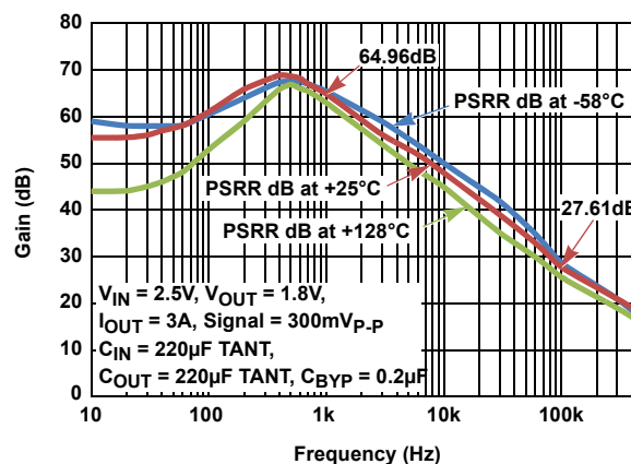
Figure 22. PSRR
