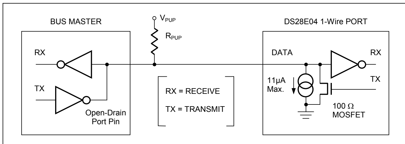
Figure 13. Hardware Configuration
