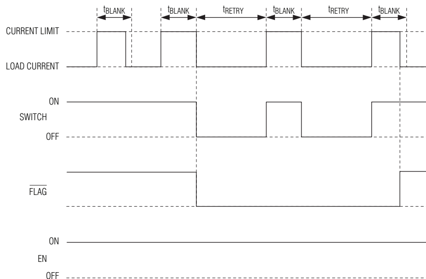
Figure 1. MAX14544 Timing Diagram (Waveforms Not to Scale)
