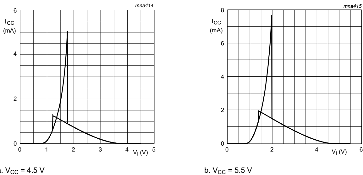
Fig. 9. Typical 74AHCT14 transfer characteristics
