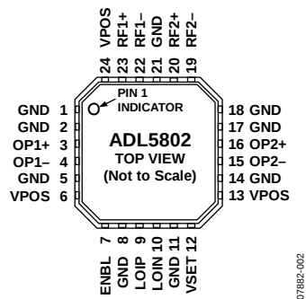
Figure 2. Pin Configuration
