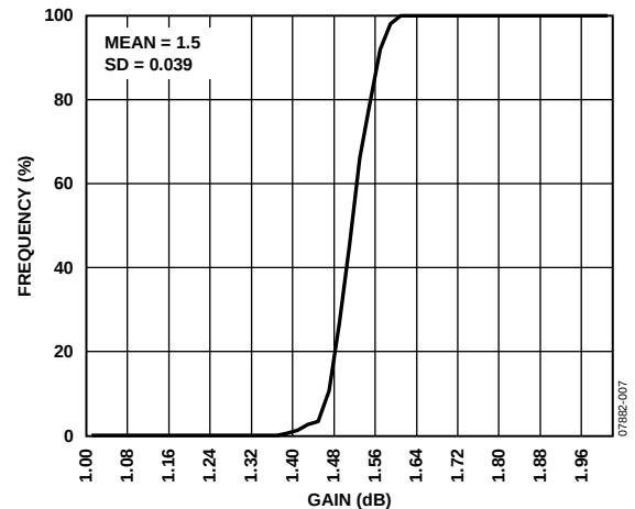
Figure 7. Power Conversion Gain Distribution
