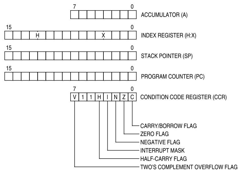
Figure 4-1. CPU Registers
