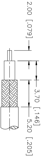
RECOMMENDED CABLE STRIPPING DIM'S
