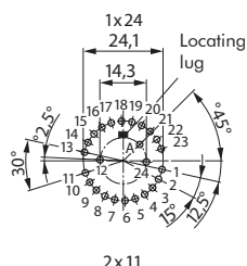
Drilling diagram 15° for indexing angle
