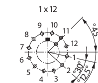
Drilling diagram 30° for indexing angle
