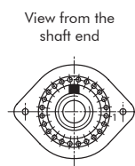
Drilling diagram 15° for indexing angle
