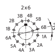
Drilling diagram 30° for indexing angle
