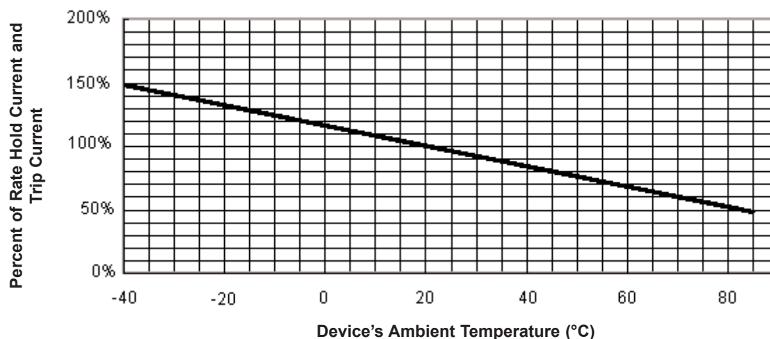
Thermal Derating Curve
