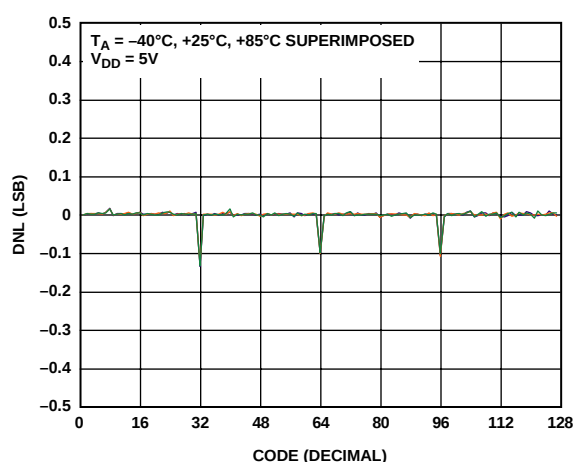
Figure 9. DNL—7-Bit RDAC
