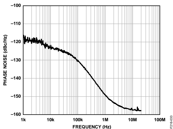
Figure 30. Phase Noise (Absolute) Clock Generation; Internal VCO at 1.966 GHz; PFD = 15.36 MHz; LBW = 40 kHz; LVPECL Output = 122.88 MHz
