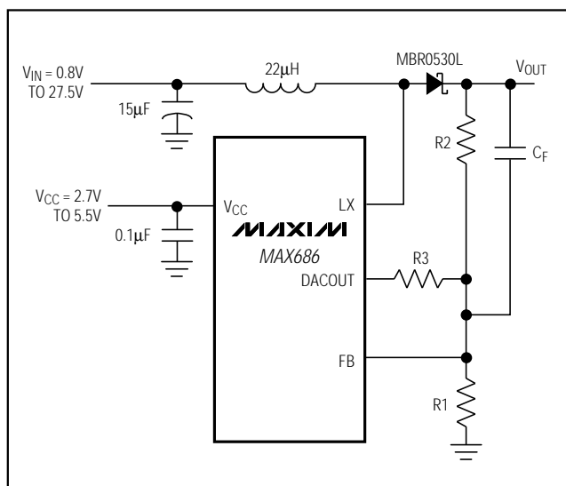
Figure 4. Feed-Forward Capacitor
