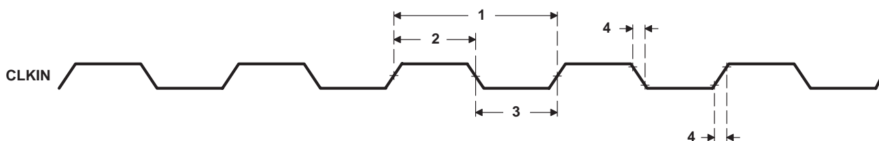
Figure 22. CLKIN Timings
