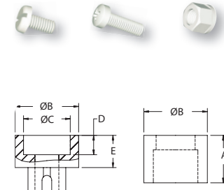
Typical Assembly
