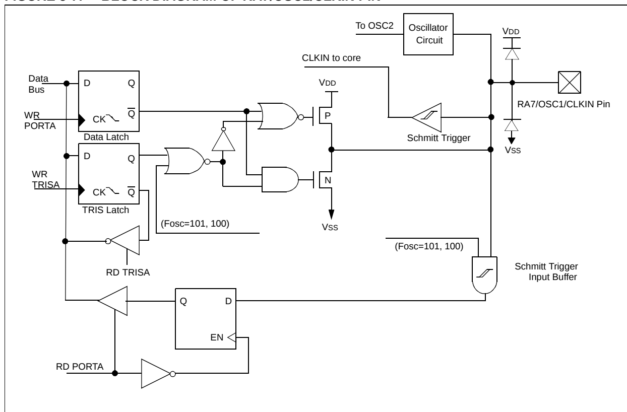
FIGURE 5-7: BLOCK DIAGRAM OF RA7/OSC1/CLKIN PIN
