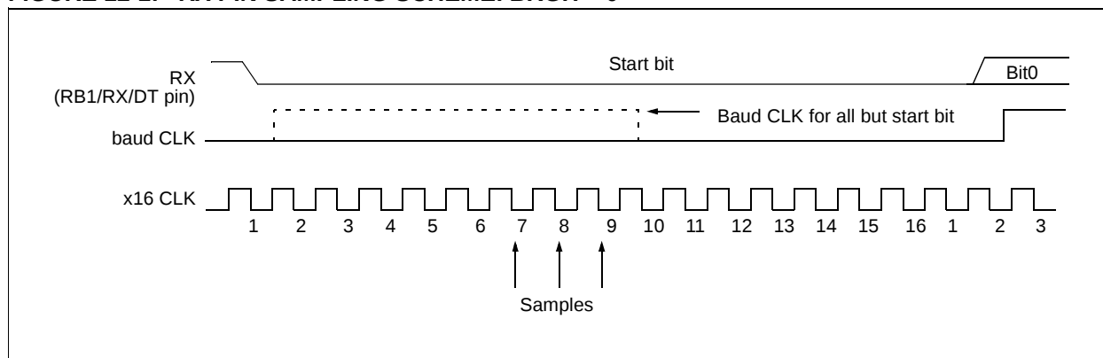
FIGURE 12-1: RX PIN SAMPLING SCHEME. BRGH = 0
