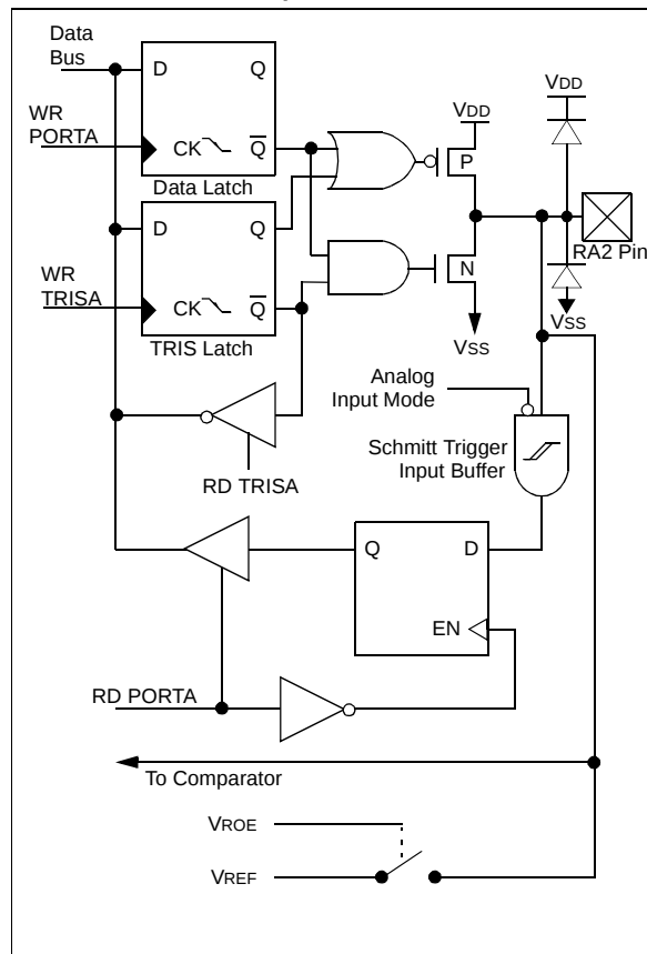
FIGURE 5-2: BLOCK DIAGRAM OF RA2/VREF PIN
