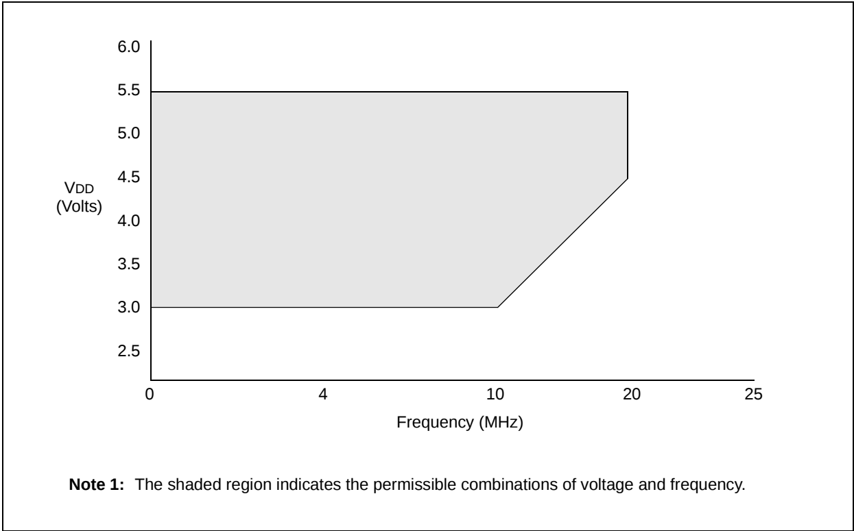
FIGURE 17-2: PIC16F62X VOLTAGE-FREQUENCY GRAPH, -40°C ≤ TA < 0°C, +70°C < TA ≤ 85°C
