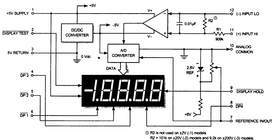
Figure 1. DMS-40PC Series Simplified Schematic
