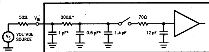
FIGURE 6. ADC08061 and ADC08062 Equivalent Input Circuit Model
