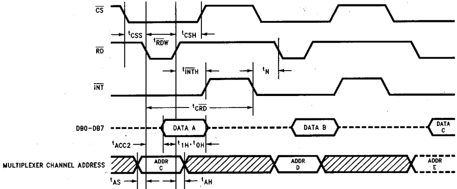
FIGURE 4. \overline{RD} Mode (Pipeline Operation) (Mode Pin is Low and t_{RDW} must be between 200 ns and 400 ns)
