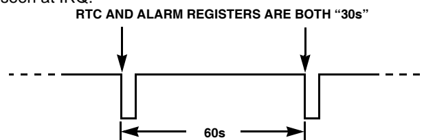
FIGURE 13. \overline{\text{IRQ}} WAVEFORM
