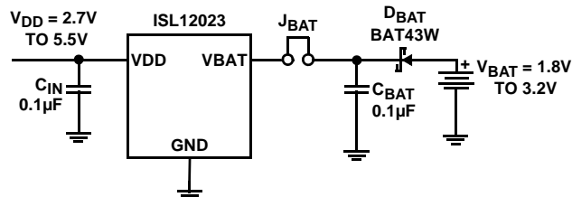
FIGURE 19. SUGGESTED BATTERY-BACKUP CIRCUIT
