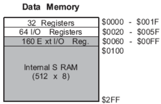
Data Memory Map
