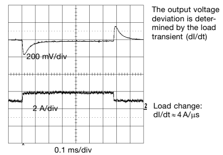
Dynamic load response (typ) @ +25^\circ\text{C}
