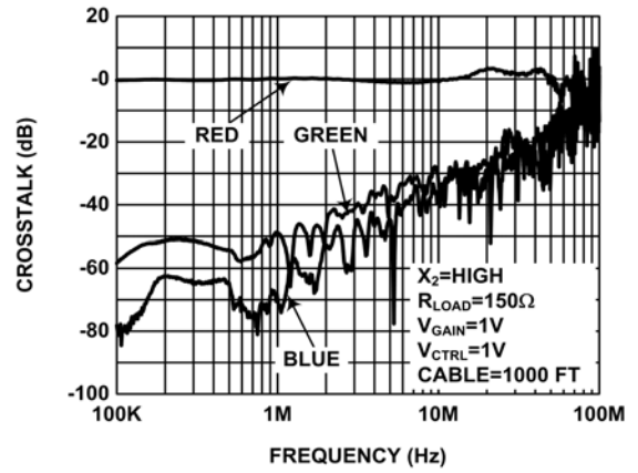
FIGURE 20. RED CROSSTALK
