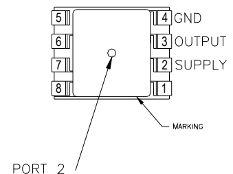
MS4525-MMvxxxxP
