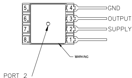
MS4525-MMvxxxxL
