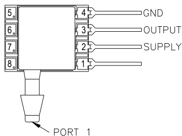
MS4525-SSvxxxxL
