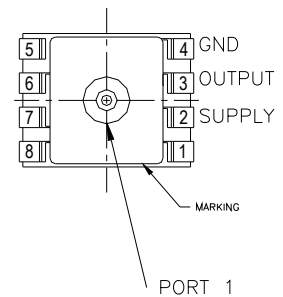
MS4525-TPvxxxxP
