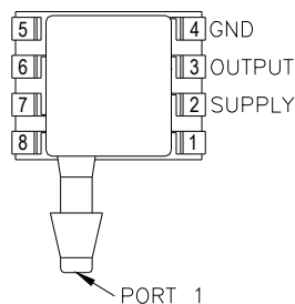
MS4525-SSvxxxxP
