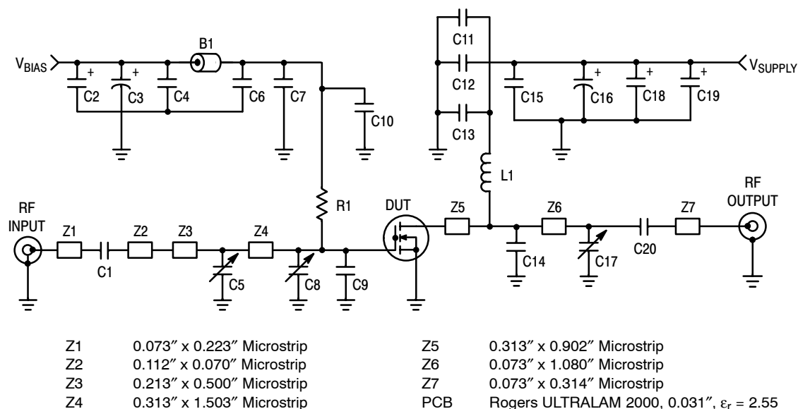
Figure 1. MW6S010MR1(GMR1) Test Circuit Schematic — 900 MHz
