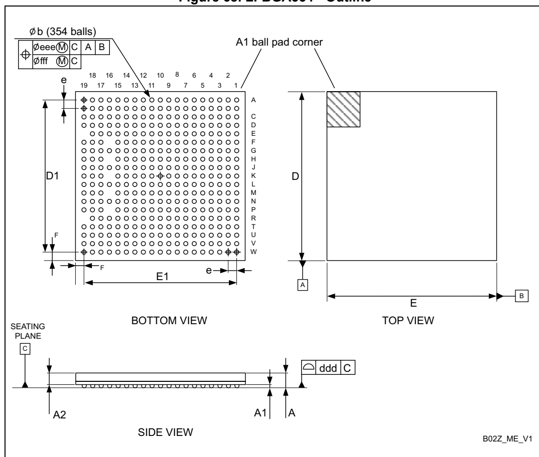
Figure 68. LFBGA354 - Outline
