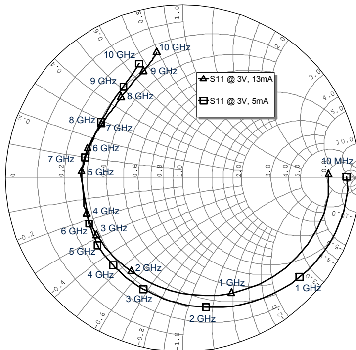
Figure 9 Input Matching S_{11} = f(\text{freq}) , V_{CE} = 3 \text{ V} , I_C = 5 \text{ mA} / 13 \text{ mA}
