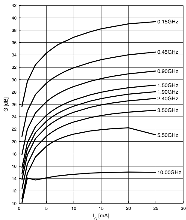
Figure 7 Power Gain G_{ma} , G_{ms} = f(I_C) , V_{CE} = 3\text{ V} , f = \text{Parameter in GHz}
