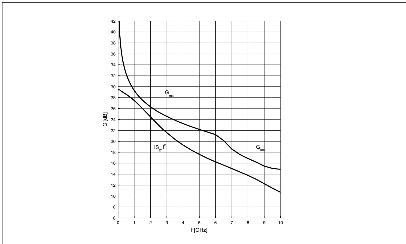
Figure 6 Power Gain G_{ma} , G_{ms} , |S_{21}|^2 = f(\text{freq}) , V_{CE} = 3 V, I_C = 13 mA
