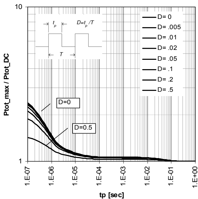
Figure 2 Permissible Pulse Load P_{\text{tot\_max}} / P_{\text{tot\_DC}} = f(t_p)
