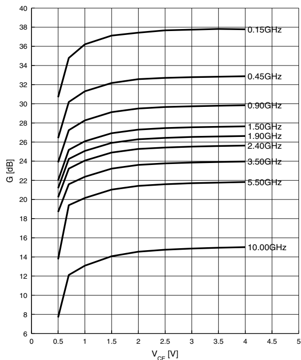
Figure 8 Power Gain G_{ma} , G_{ms} = f(V_{CE}) , I_C = 13\text{ mA} , f = \text{Parameter in GHz}
