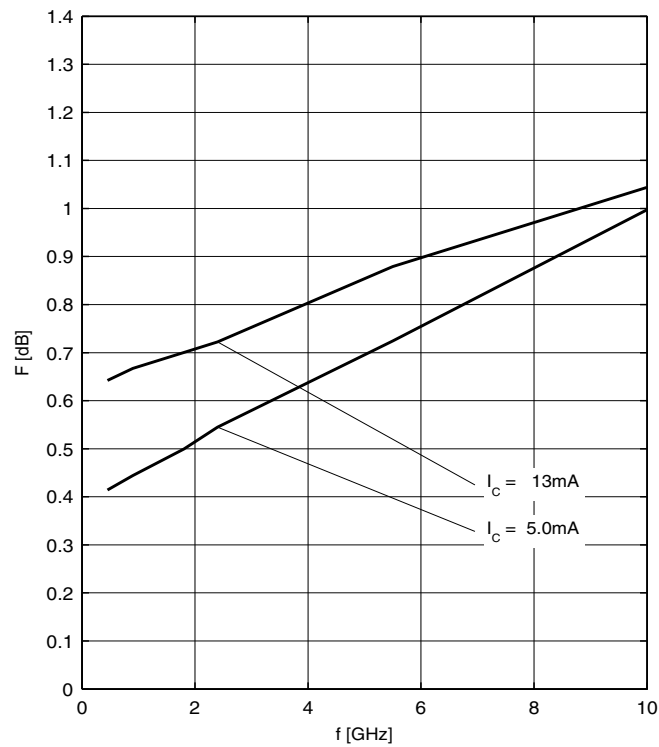
Figure 13 Noise Figure NF_{\min} = f(\text{freq}) , V_{CE} = 3\text{ V} , Z_S = Z_{\text{opt}}
