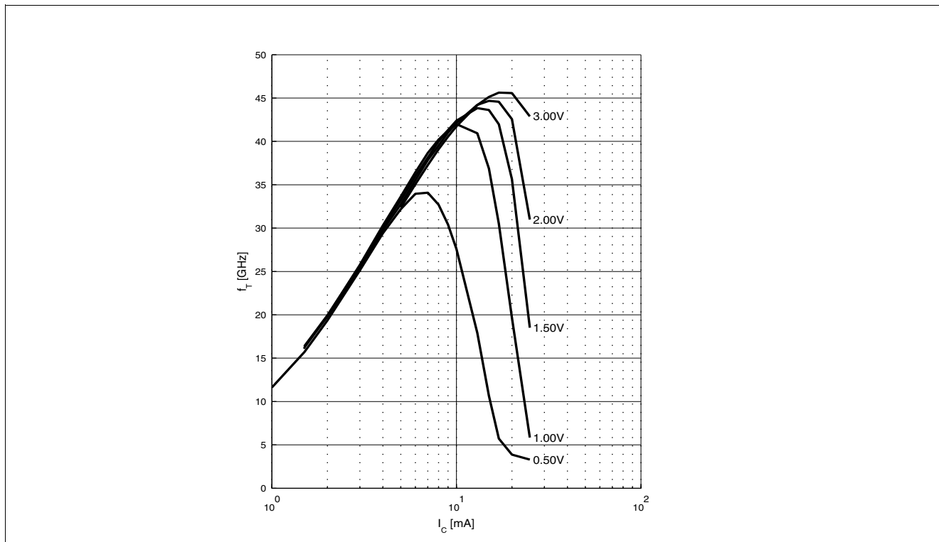
Figure 5 Transition Frequency f_T = f(I_C, V_{CE}) , f = 1 GHz, V_{CE} Parameter in V
