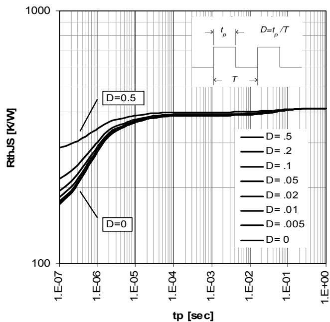
Figure 3 Permissible Pulse Load R_{\text{thJS}} = f(t_p)
