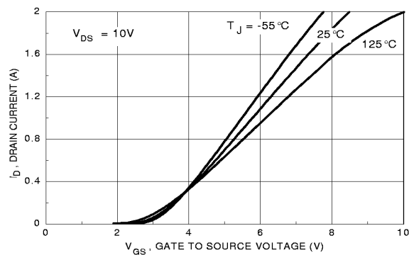
Figure 5. Transfer Characteristics
