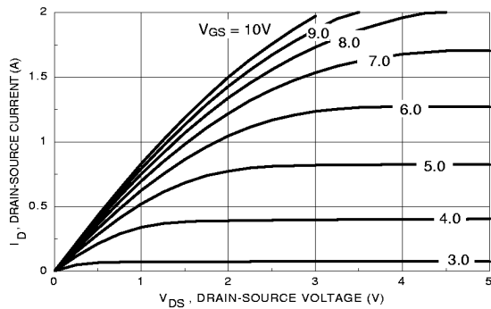
Figure 1. On-Region Characteristics
