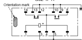
Terminal Arrangement/Internal Connections (Top View) G6Z-1F-A
