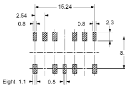
Mounting Dimensions (Top View) Tolerance: \pm 0.1 mm
