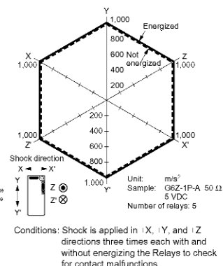
Shock Malfunction
