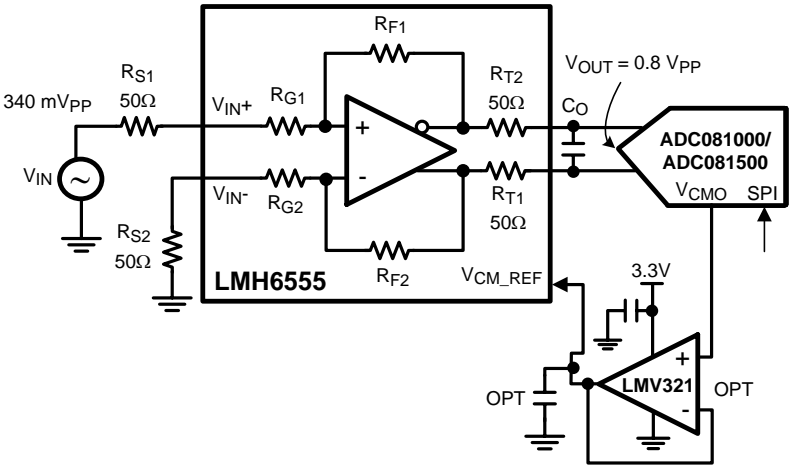
Figure 41. Increasing ±0.5 dB Gain Flatness using External Output Capacitance, C O
