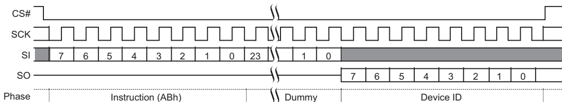
Figure 9.26 Read Electronic Signature (RES ABh) Command Sequence
