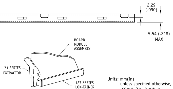
71 SERIES EXTRACTOR
