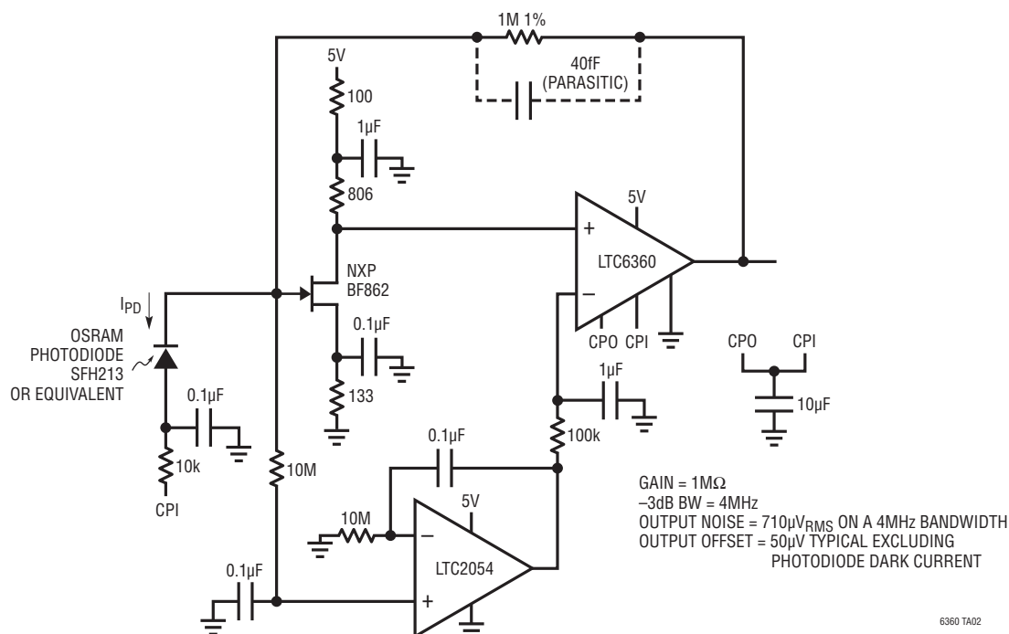
Precision Ultralow Noise True Zero Photodiode Amplifier
