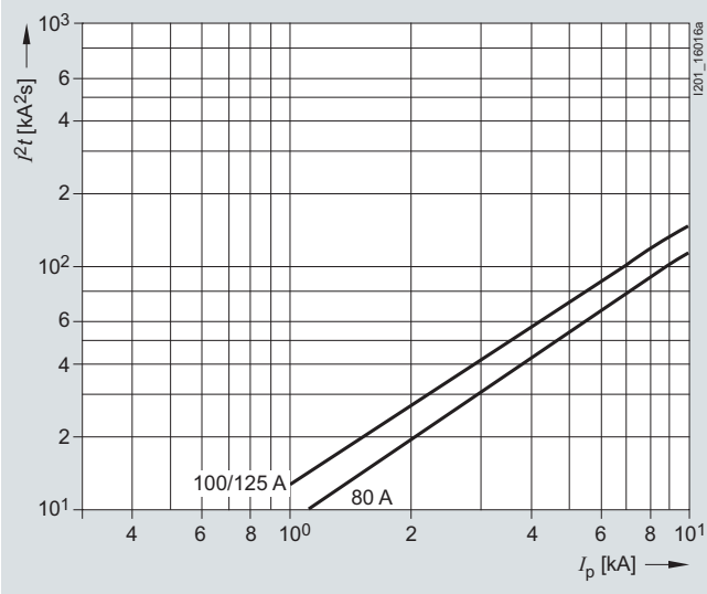
Characteristic B
